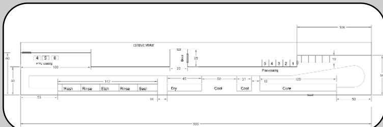
Single turn production line provides efficient powder coating of long parts.
